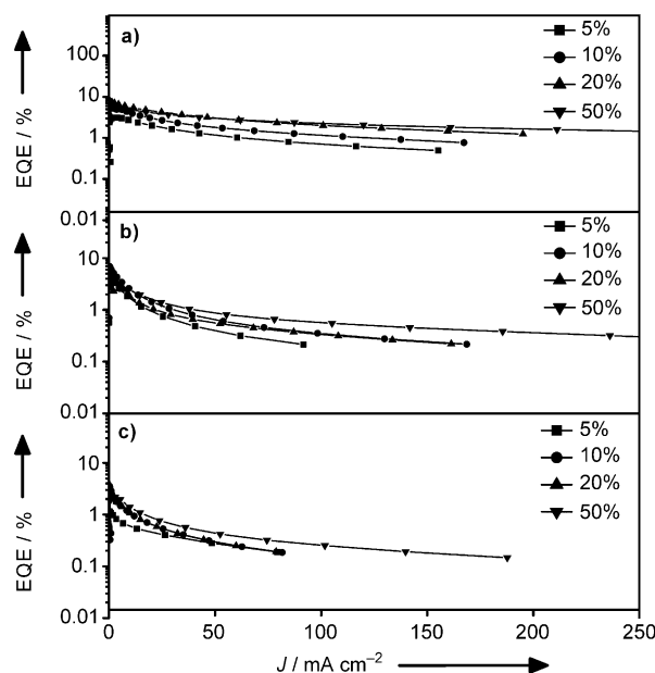
Figure 2. EQE of the devices with a) 1 , b) 2 , and c) 3 doped into MCP as the light-emitting layer.
