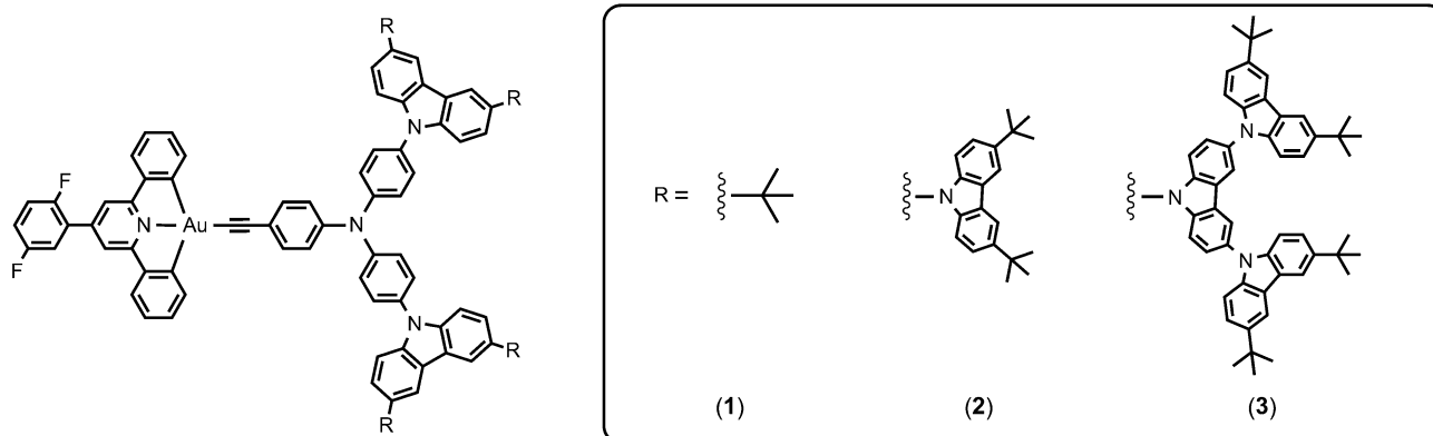
Scheme 1. Chemical structures of the alkynylgold(III) dendrimers 1–3 .
